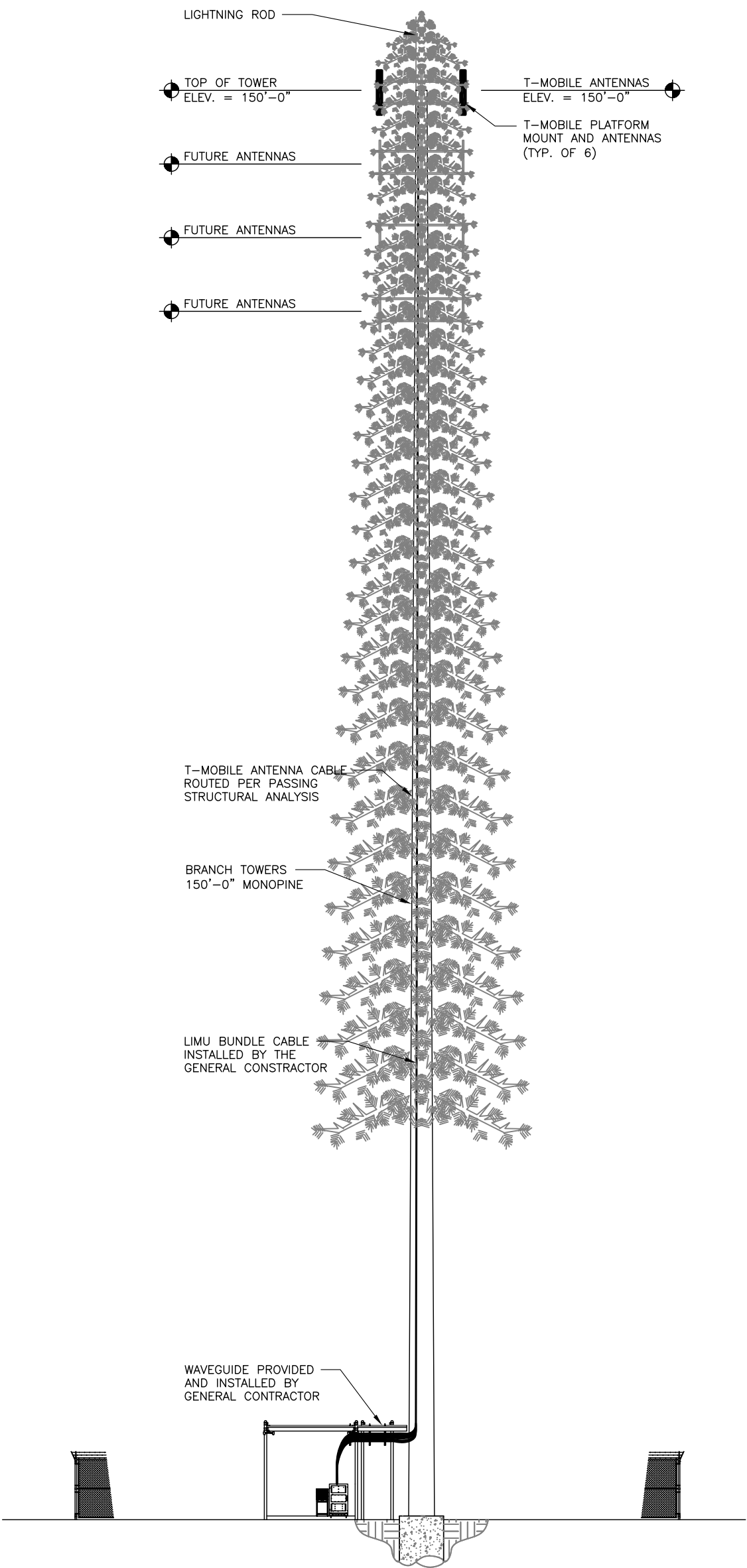
1 PROPOSED TOWER ELEVATION SCALE: N.T.S.
